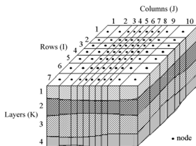
Figure 2.1. Spatial discretization of an aquifer system and the cell incides
