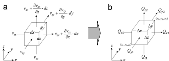
Partial Differential Approach
