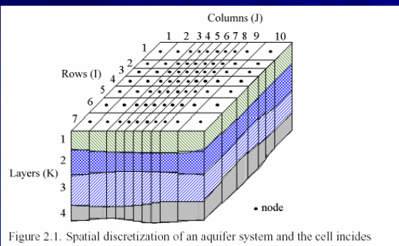
Figure 2.1. Spatial discretization of an aquifer system and the cell incides
